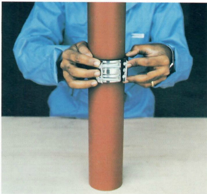
Step 5 – Place steel fastener in position over rubber seal
