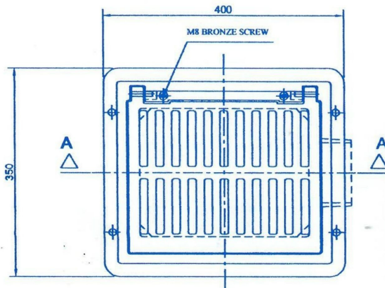
PLAN VIEW
