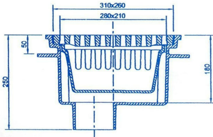
SECTION - AA (BOTTOM OUTLET)
